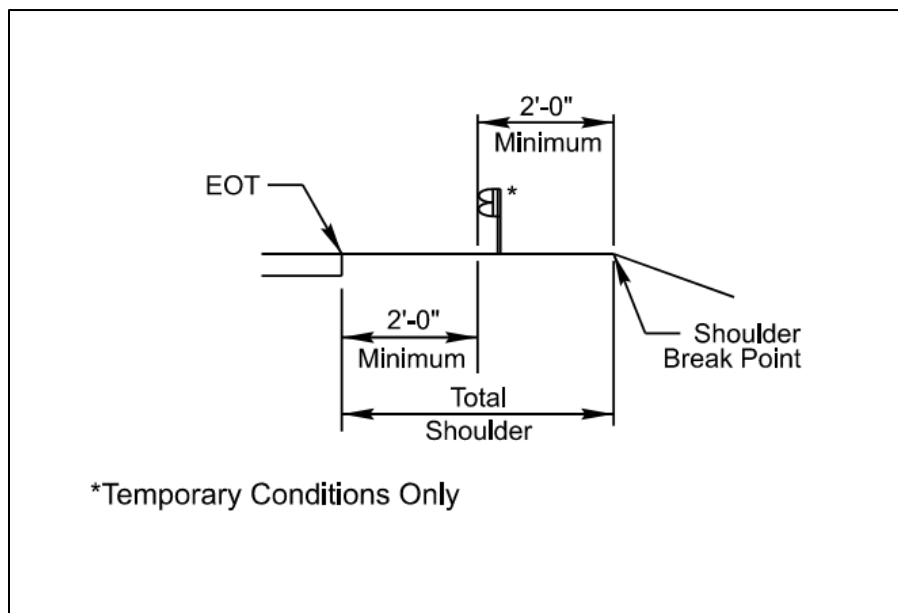
Figure 6-5 Minimum Offsets for Temporary Guardrail Placement
