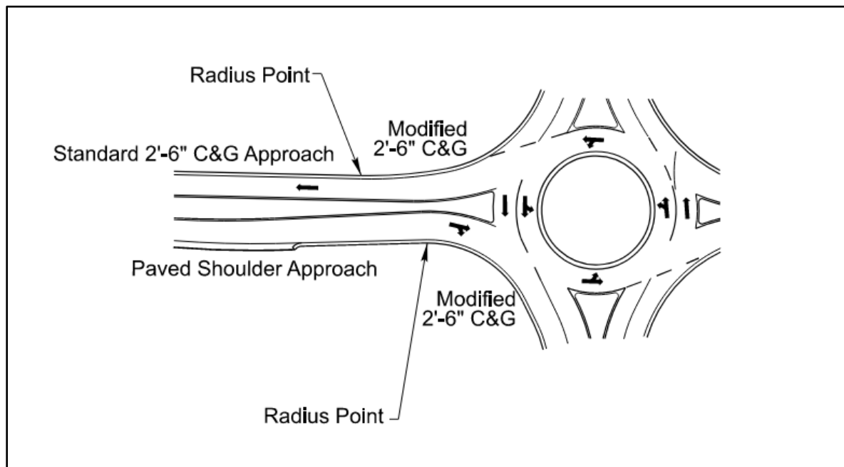
Figure 8-18 Roundabout Modified Curb and Gutter Transition
