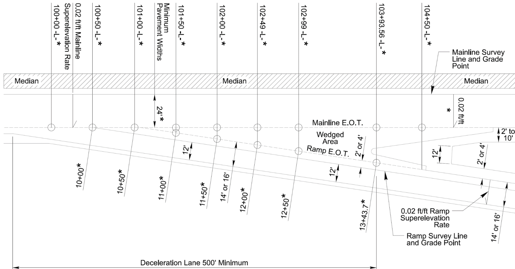
Figure 9-4 Ramp Gore Grade Control Points
