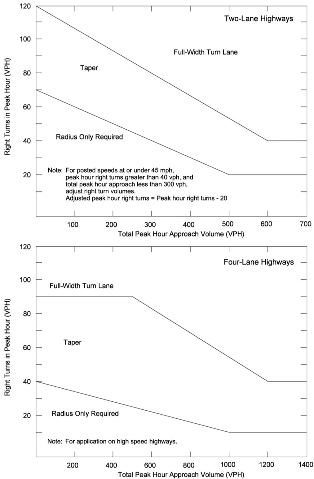
Figure 8-9 Right Turn Lane Warrants
