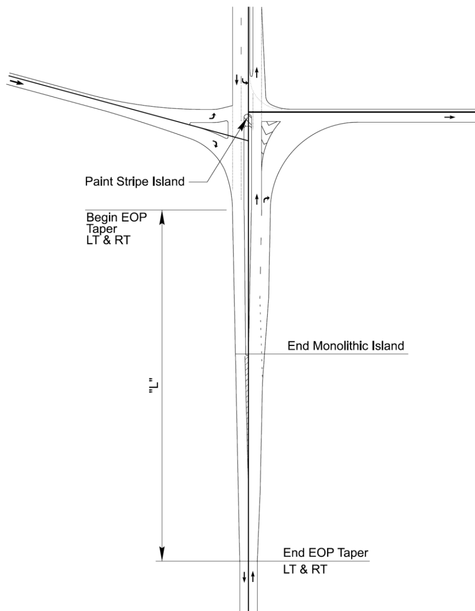
Figure 9-8a Y- Line Transition at Ramp Terminal for Three-Lane -Y- Line Section (Recommended)
