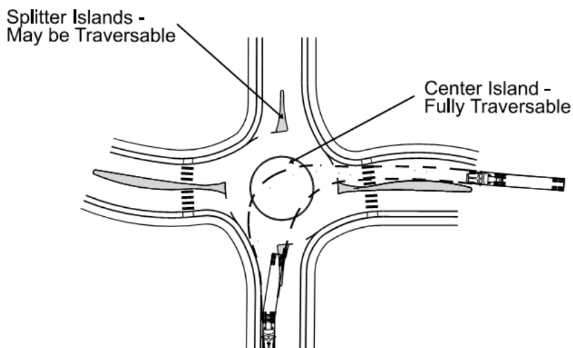
Figure 8-21 Mini-Roundabout Features
