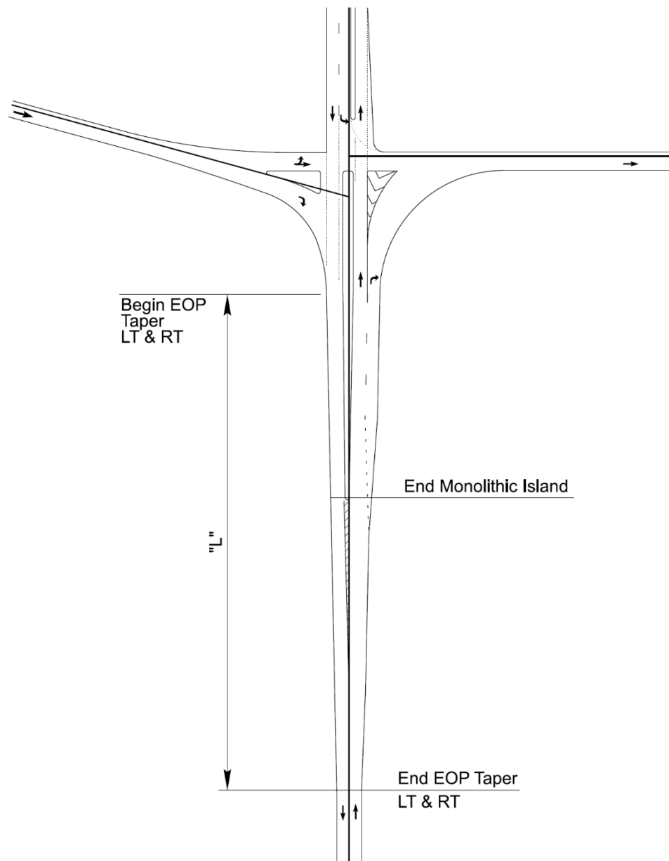
Figure 9-8b Y- Line Transition at Ramp Terminal for Three-Lane -Y- Line Section (Alternate)
