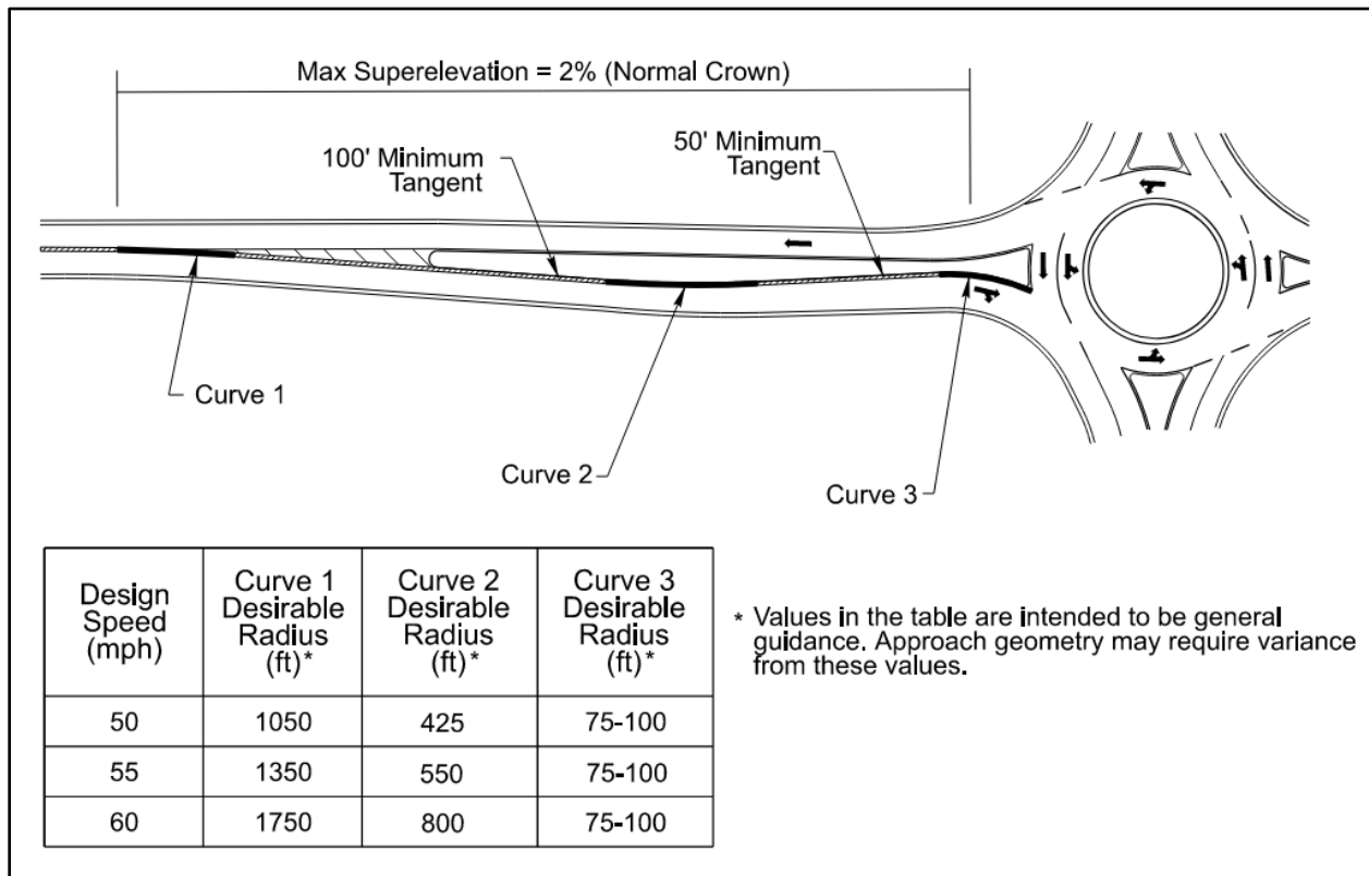
Figure 8-20 High-Speed Roundabout Approach
