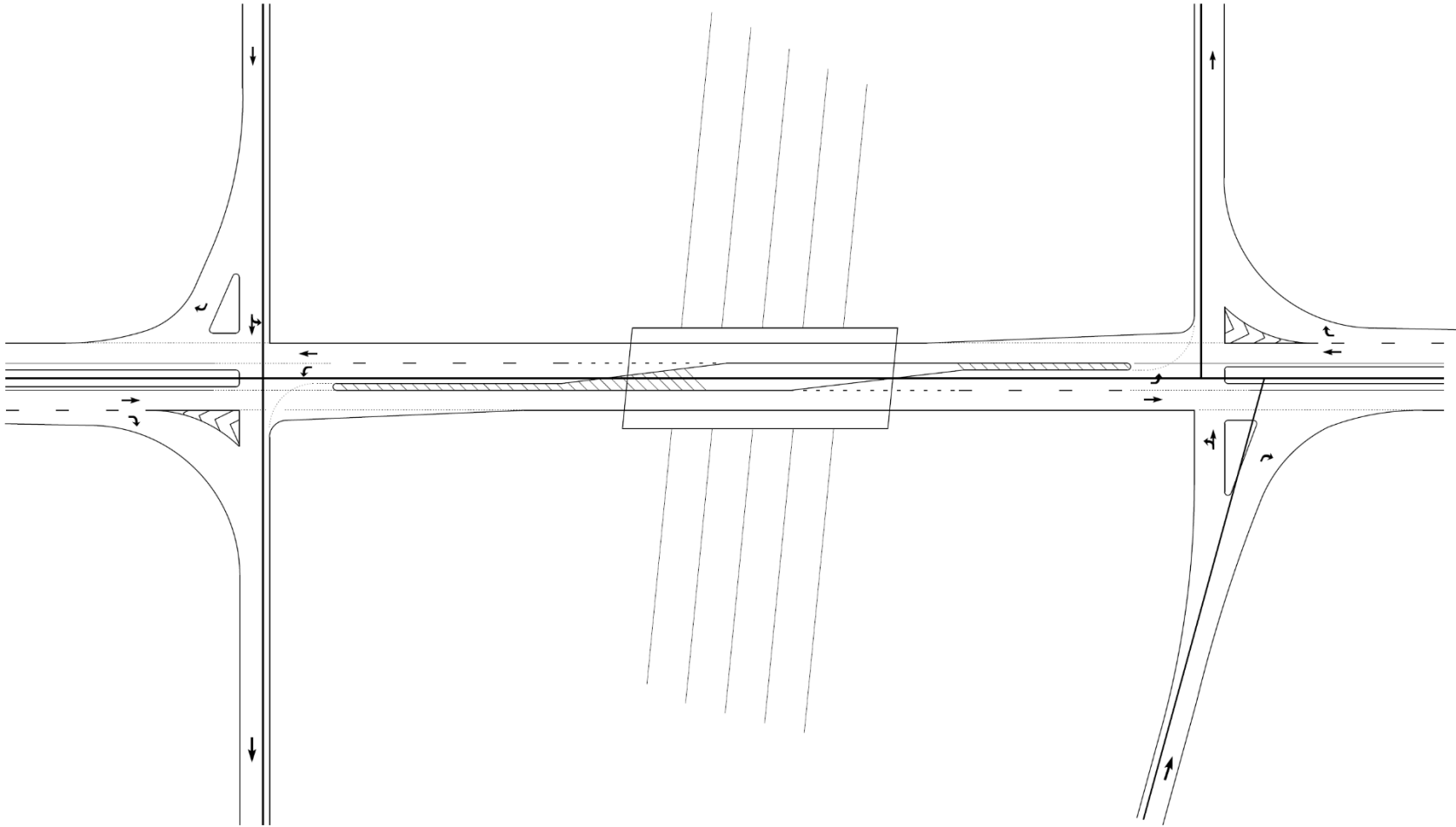
Figure 9-9b Ramp Terminal Design (Alternate)
