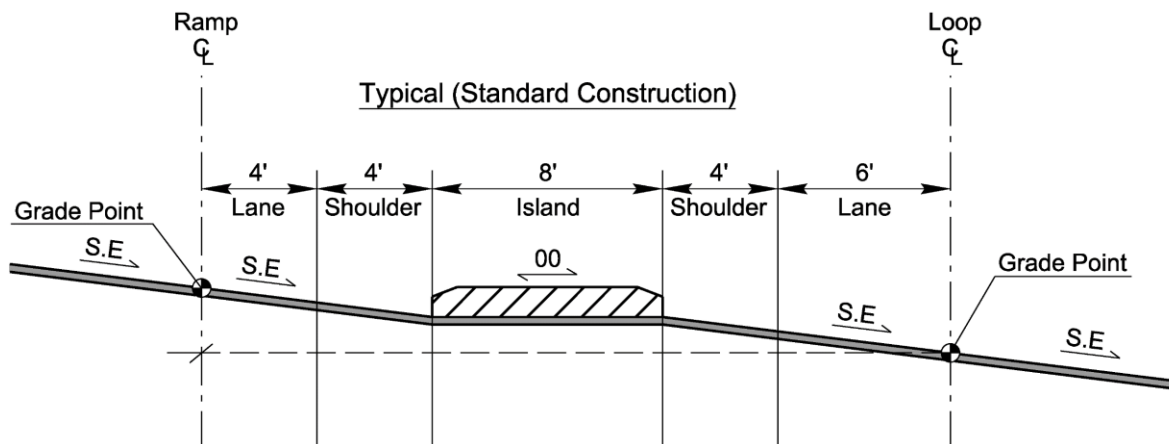
Figure 9-11 Section View for Loop Ramp Terminal Combination
