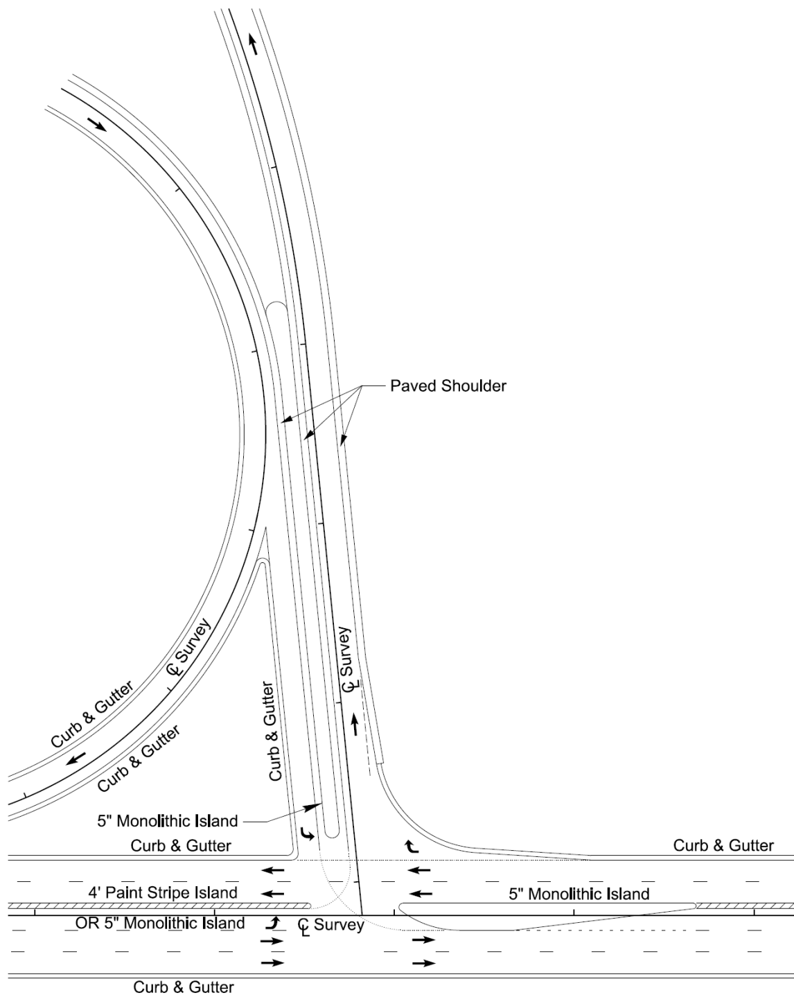
Figure 9-10 Plan for Loop Ramp Terminal Combination
