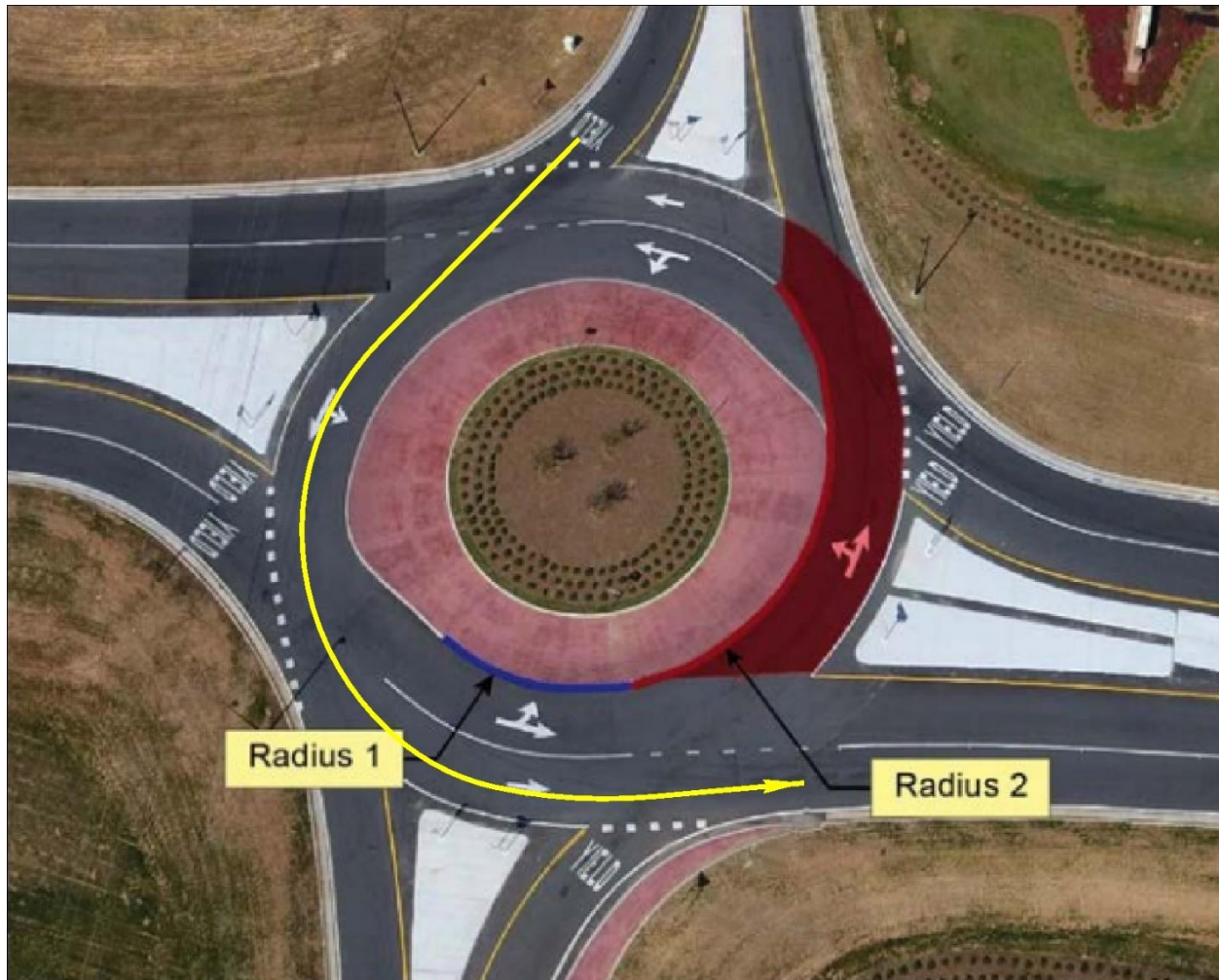
Figure 8-19 Spiraling in a 2x1 Roundabout
