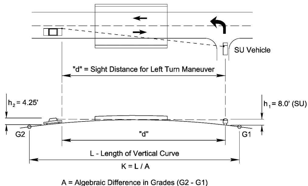
Figure 9-6 Vertical Sight Distance Control for Crest Curves at Interchanges, Single Unit Vehicle Criteria
