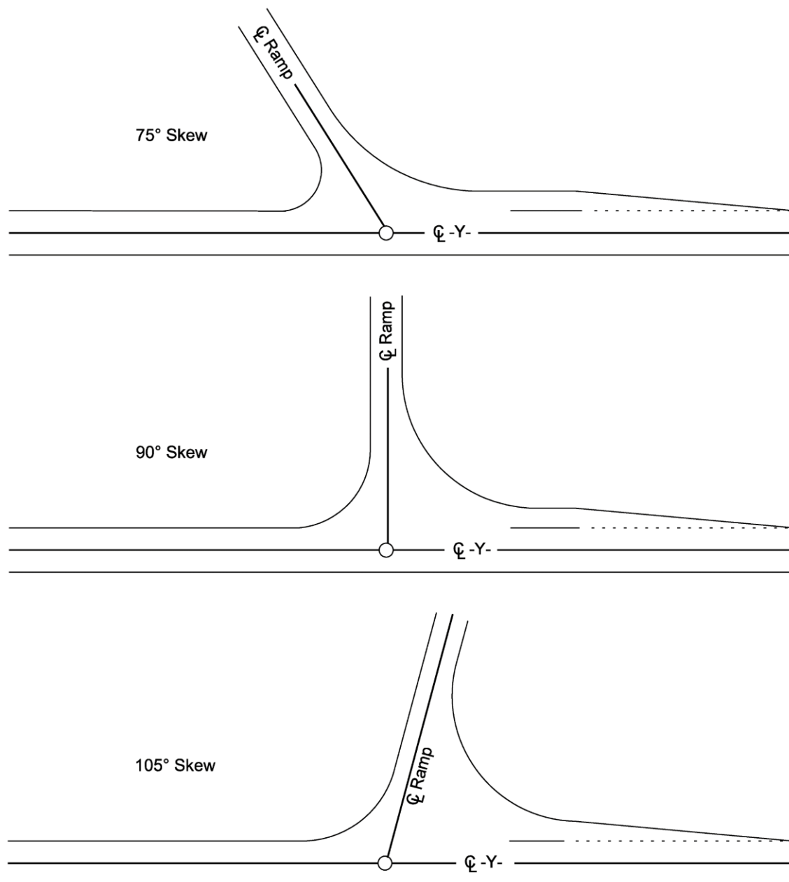
Figure 9-12 Acceptable Ramp Terminal Skews
