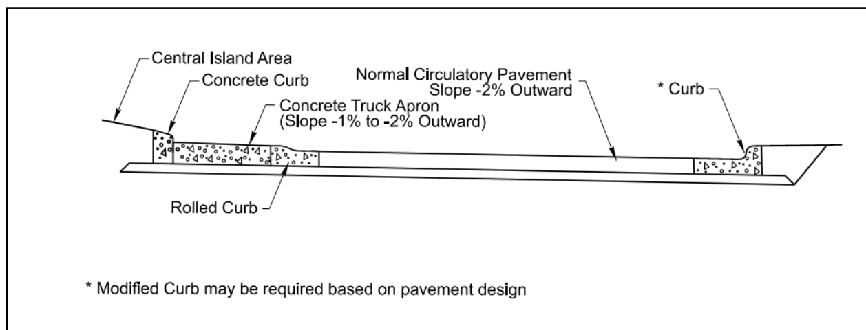
Figure 8-17 Example Roundabout Typical Section
