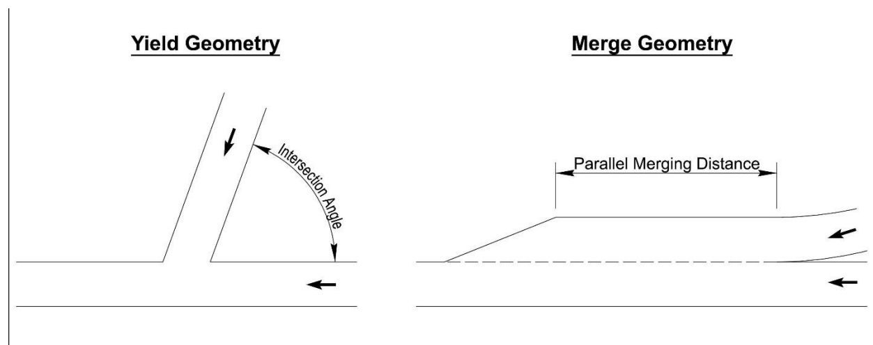
Figure 9-3 Merging and Yielding Geometry
