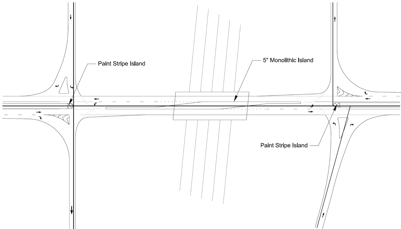
Figure 9-9a Ramp Terminal Design (Recommended)
