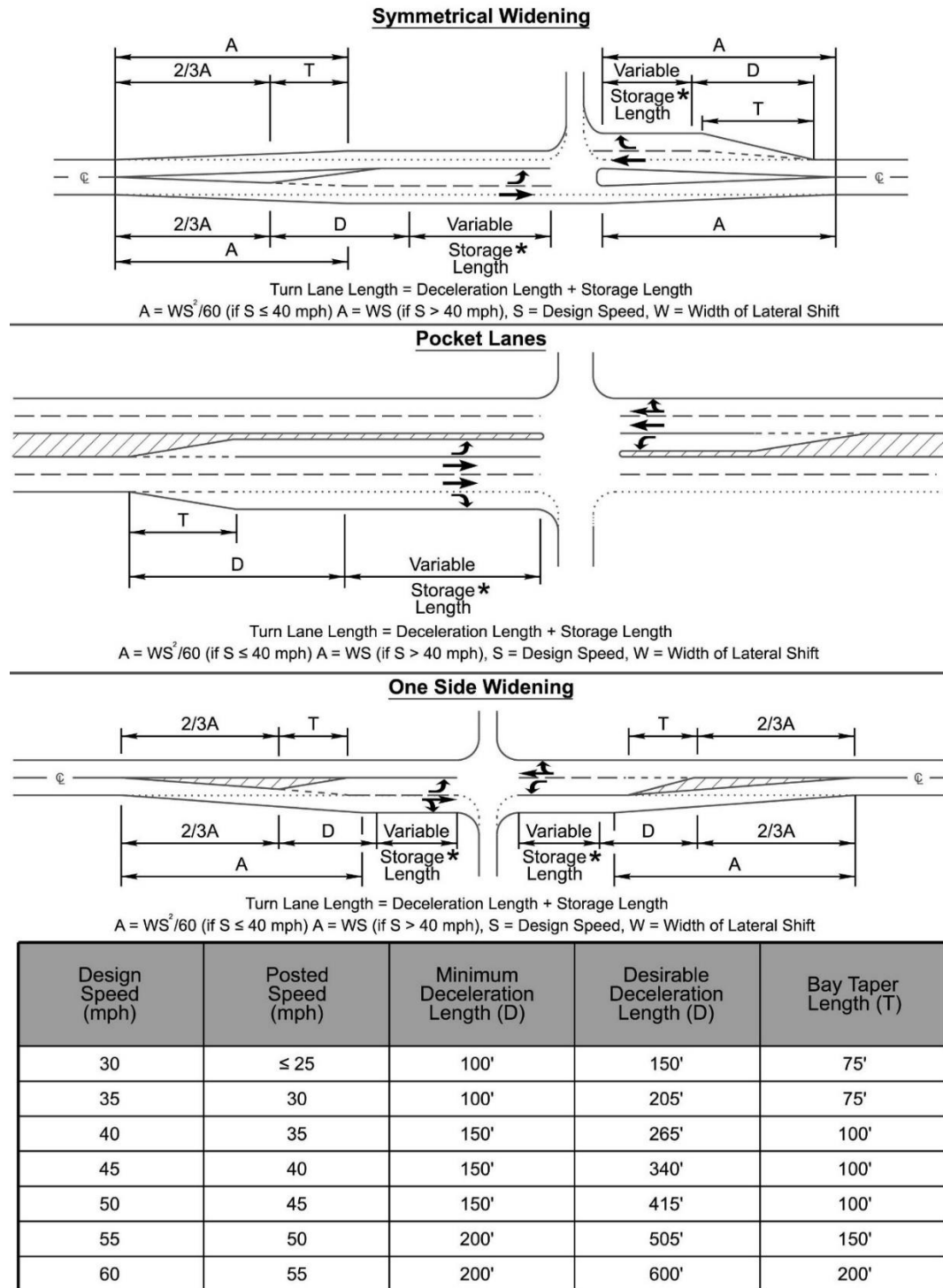
Figure 8-11 Recommended Treatment for Turn Lanes
